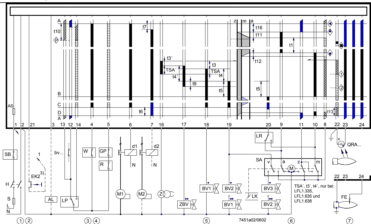
Connection diagram
